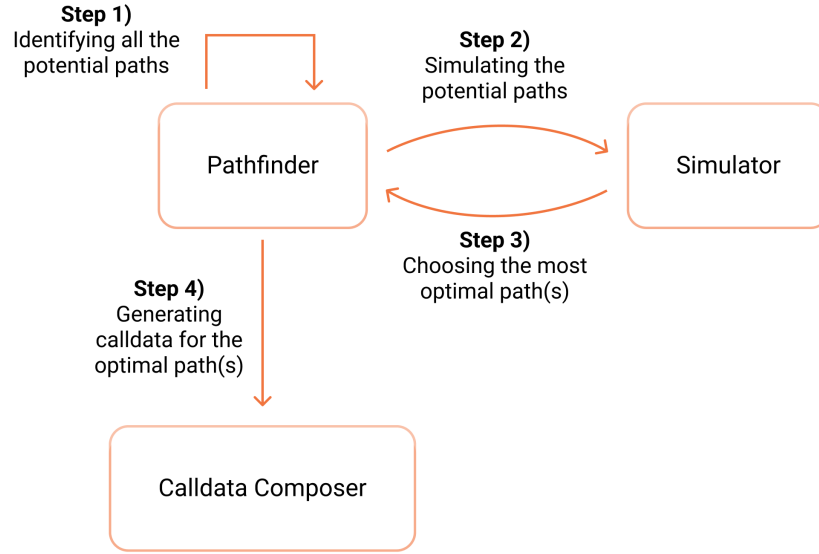
Figure 3: Intent Solver Workflow
